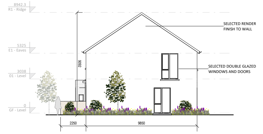
③ H01 Exposed Gable Condition 1 : 200
