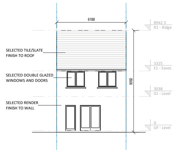
④ H01 Rear Elevation 1 : 200
