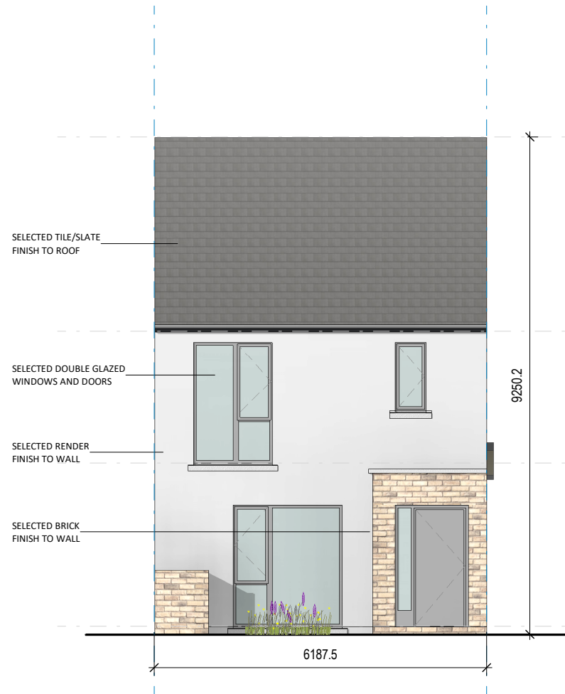
① H01 Front Elevation 1 : 100
