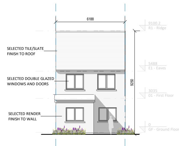
⑤ H01 Rear Elevation (Extended) 1 : 200
