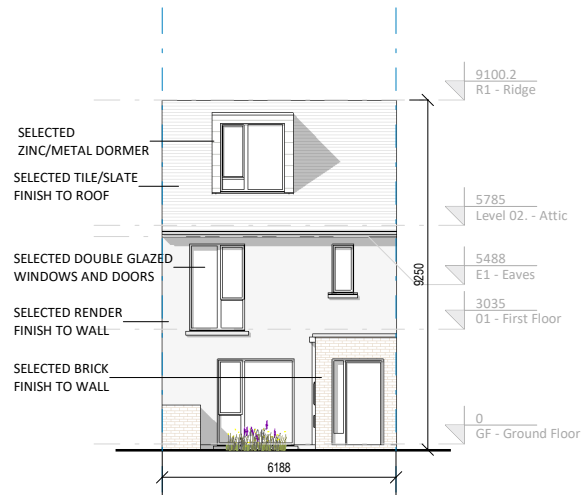
② H01 Front Elevation with Attic Conversion 1 : 200
